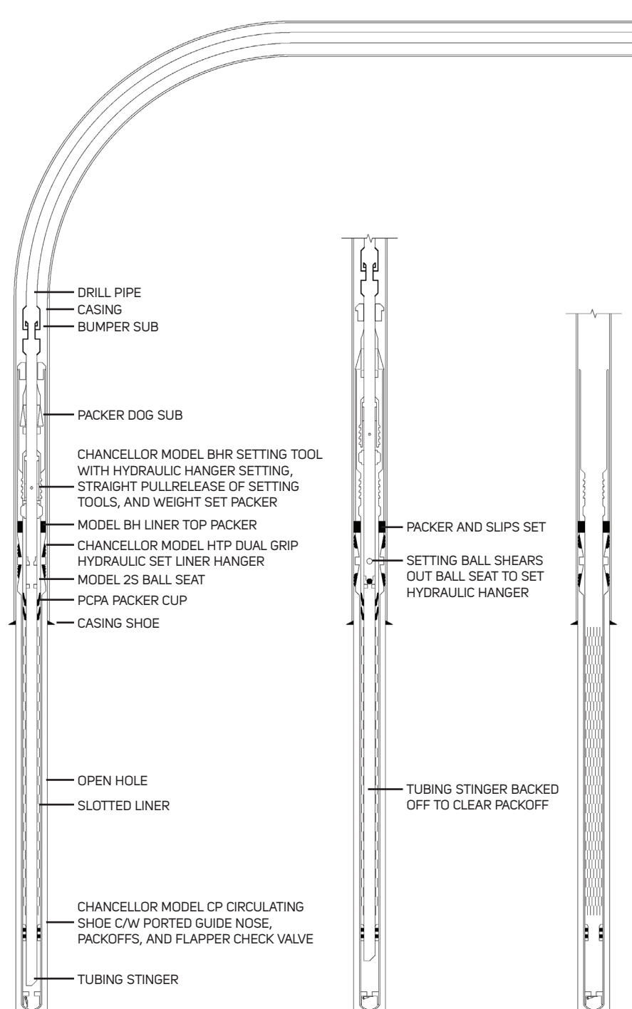
LINER ON BOTTOM CIRCULATING OR PUMPING CHANGE OVER
