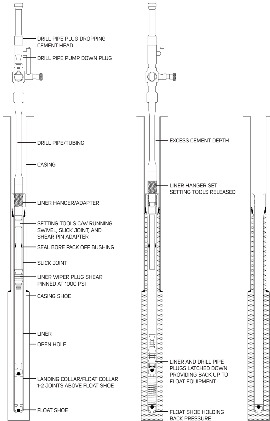
LINER ASSEMBLY ON BOTTOM CIRCULATING
