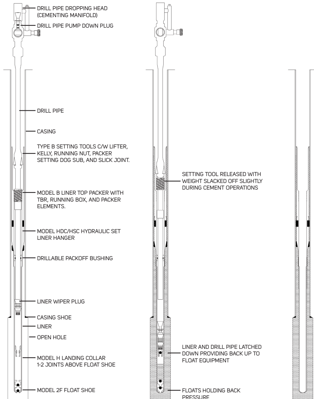
LINER ASSEMBLY ON BOTTOM CIRCULATING
